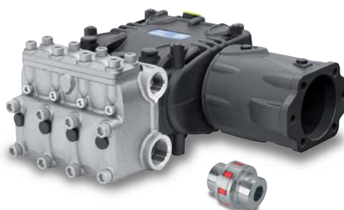
Bell housing and coupling for SAE J 744 B-B hydraulic motor
