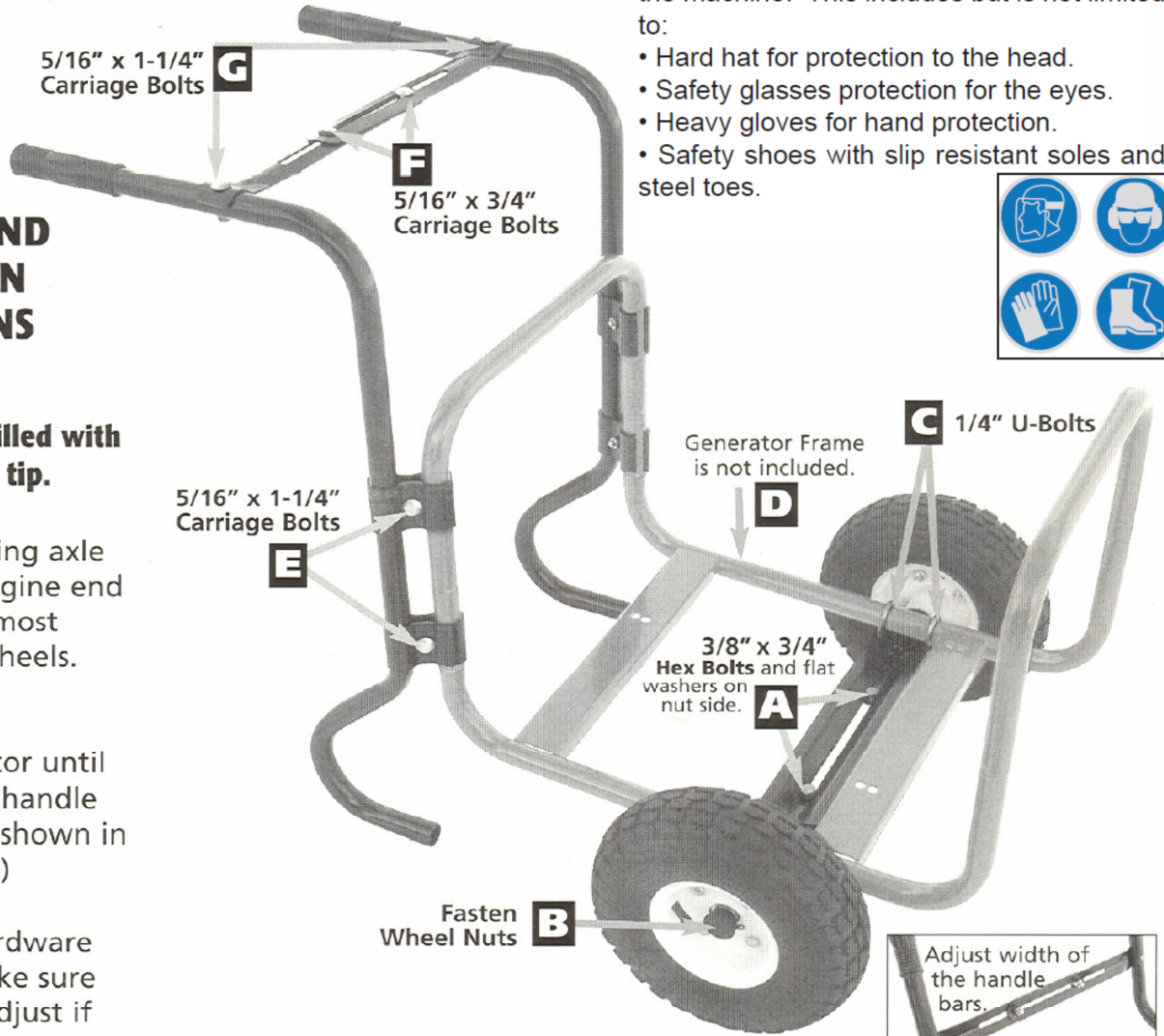
Frame of generator on axle. Place U-Bolts into provided holes.
