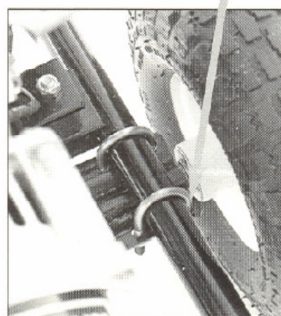
Frame of generator on axle. Place U-Bolts into provided holes.
