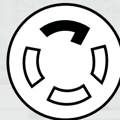
Twist lock AC NEMA L14-30R 120V/240V 30A
