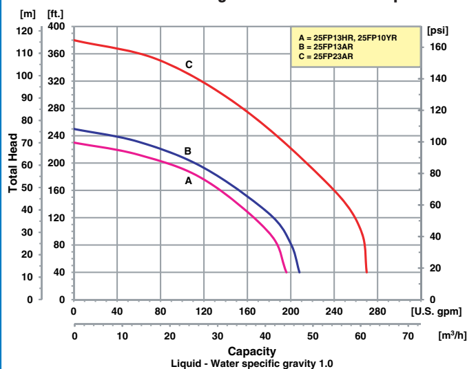
Performance of Engine Driven Fire Pumps
