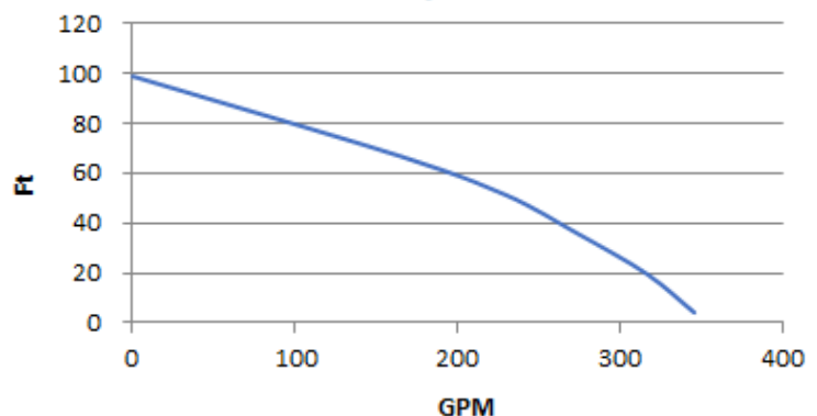
Pump Curve
