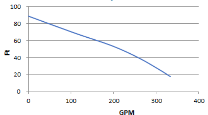
Pump Curve
