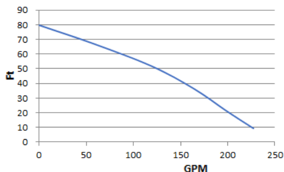
Pump Curve
