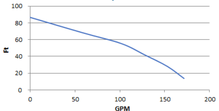
Pump Curve
