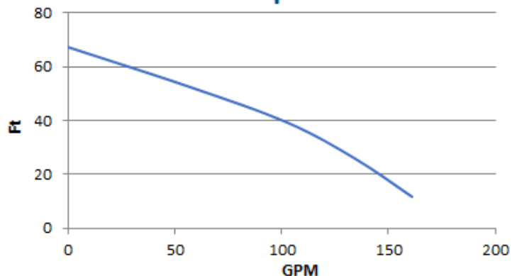
Pump Curve
