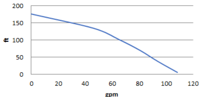
Pump Curve
