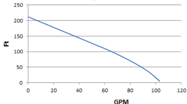
Pump Curve
