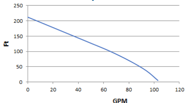
Pump Curve
