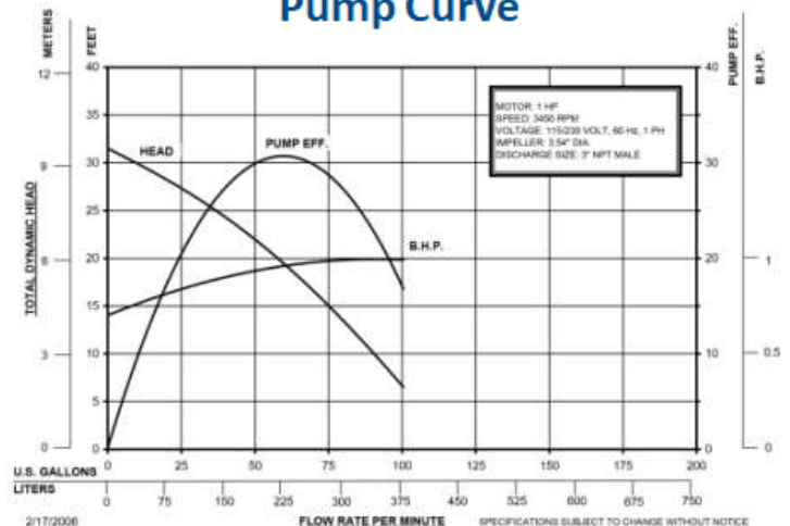
Pump Curve
