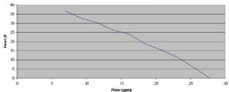
Pump Curve
